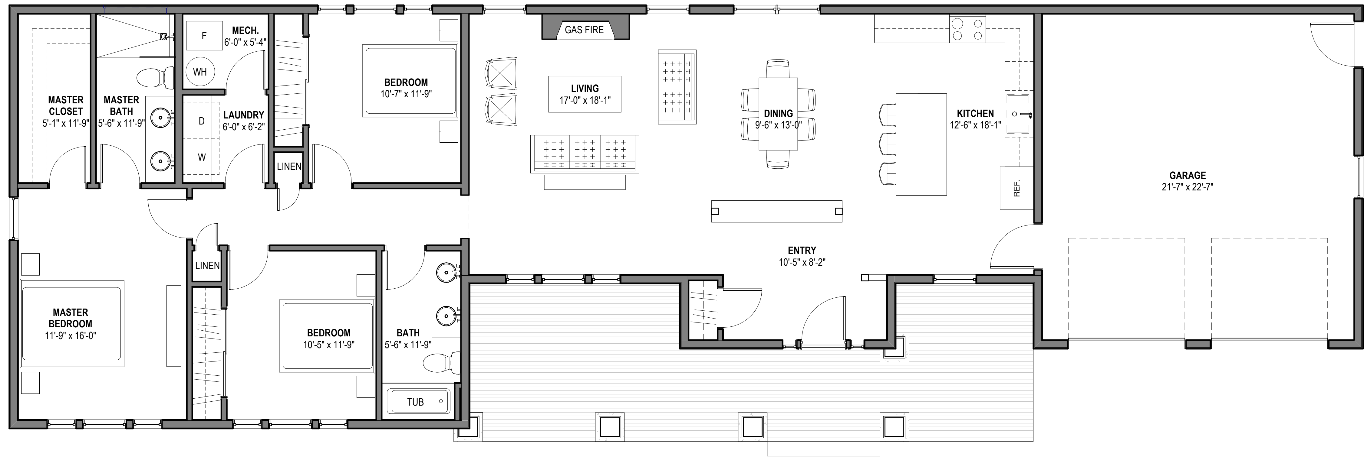
FLOOR PLAN 0' 2' 4' 8' 16'
